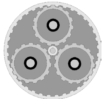
gear wheels
